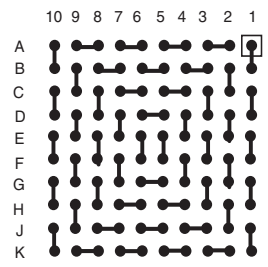
BGA100T.8-DC109
