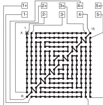
BGA225 AFTER MOUNTING TO TEST BOARD
