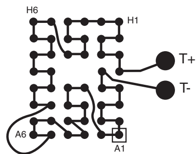
AFTER MOUNTING TO TEST BOARD
