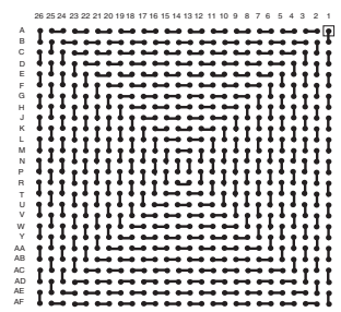
BGA676T1.0-DC269
