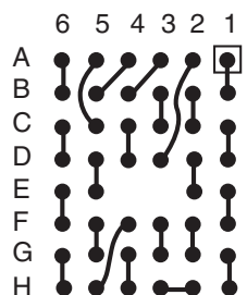
BGA46T.75-DC24
