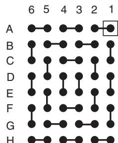
LBGA48T.8-DC689
