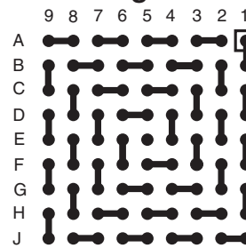
BGA81T.8-DC099
